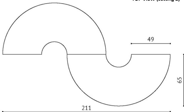
TOP VIEW (setting 2)
