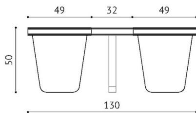
SIDE VIEW (one module)
